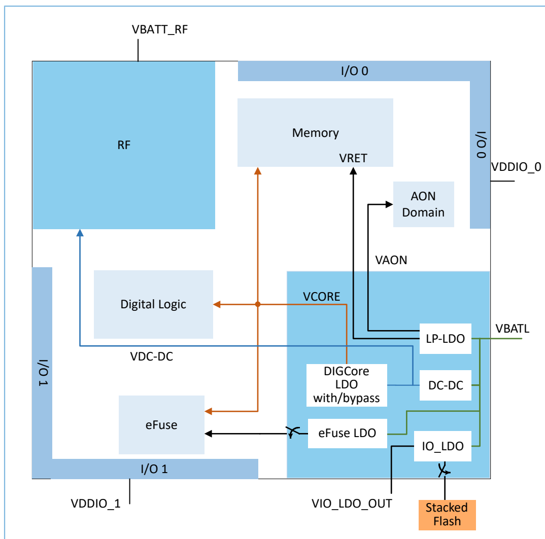
Figure 6-2 Power architecture
