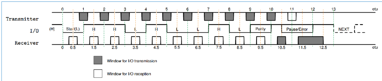
Figure 10-35 Character Timing
