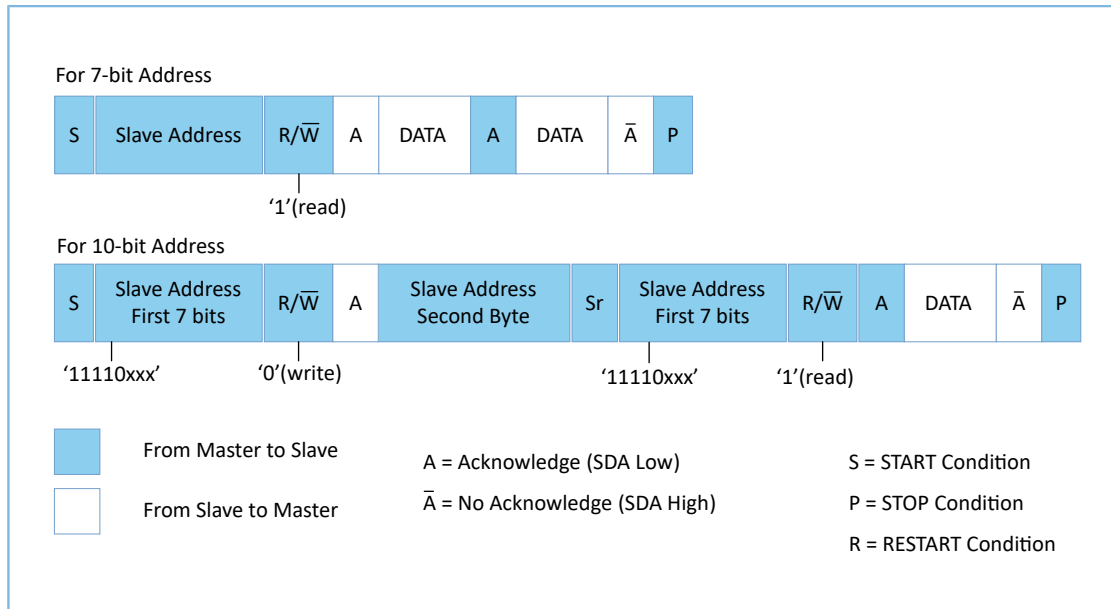
Figure 10-9 Master-Receiver Protocol
