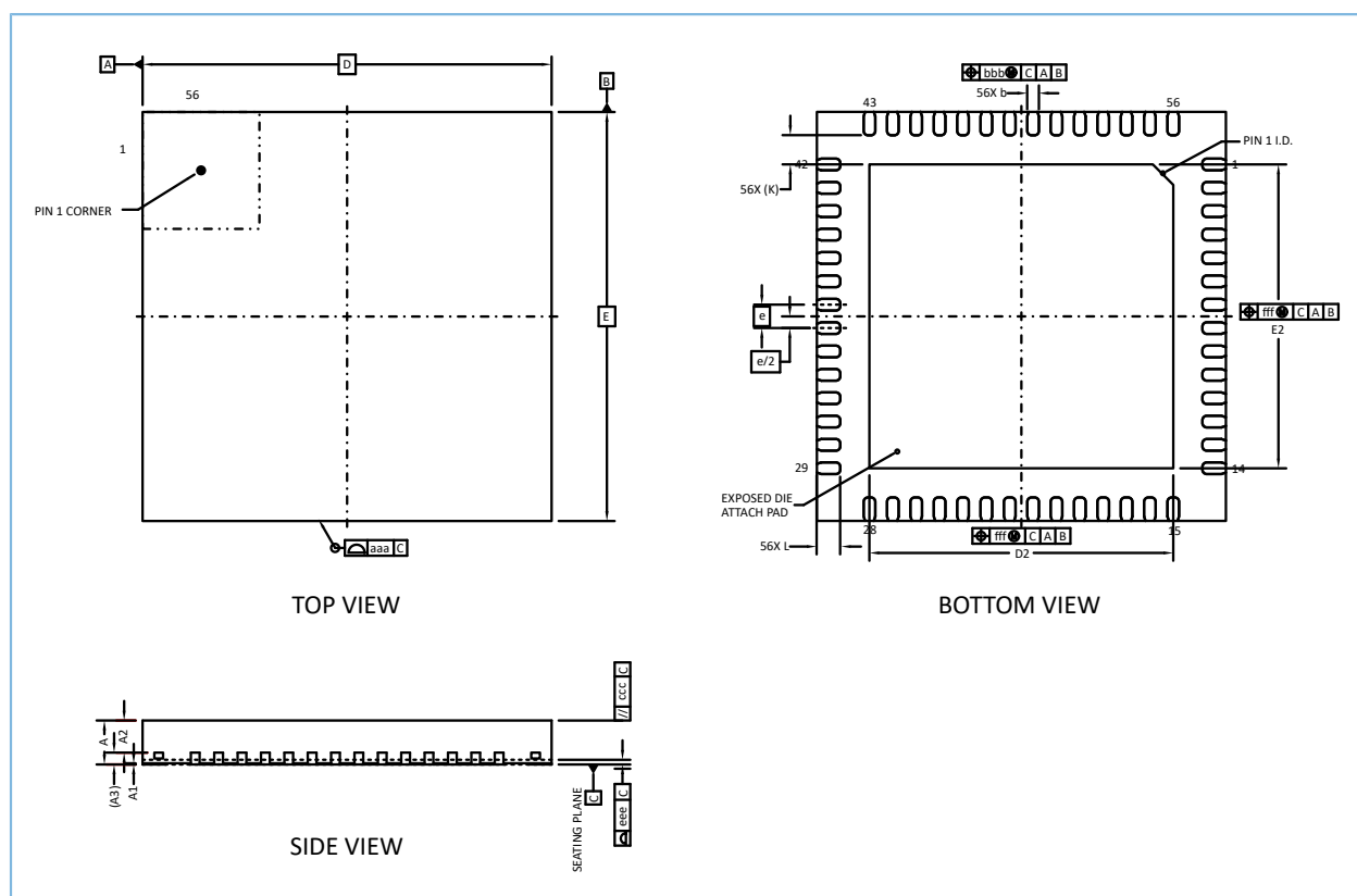
Figure 14-1 QFN56 package outlines
