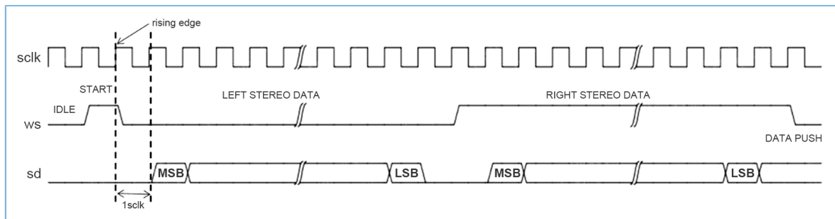
Figure 10-26 I2S formats
