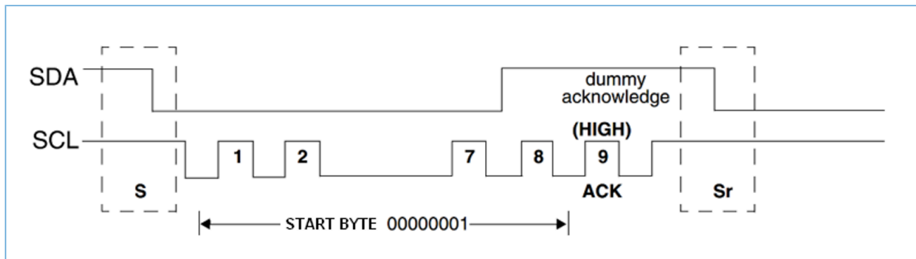
Figure 10-10 START BYTE Transfer
