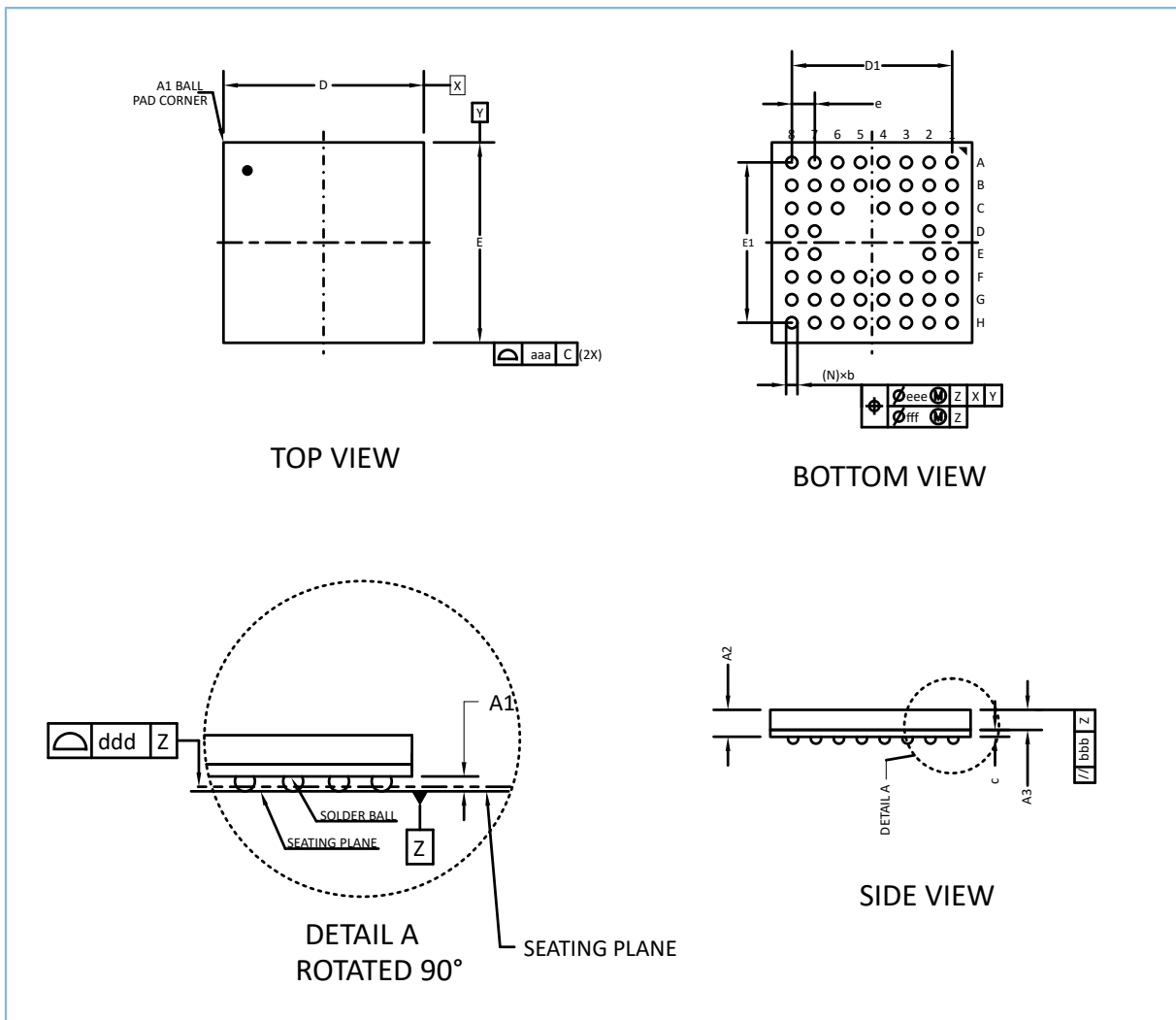
Figure 14-3 BGA55 package outlines
