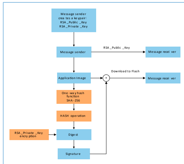
Figure 3-2 Signing process
