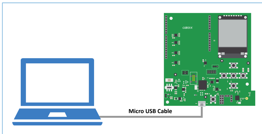
Figure 2-1 Hardware connection
