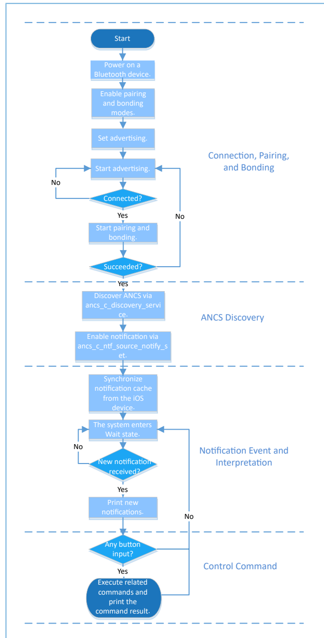
Figure 4-1 ANCS Client-Server interaction process
