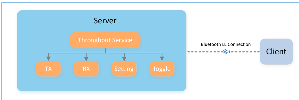
Figure 2-1 Server-client interactions
