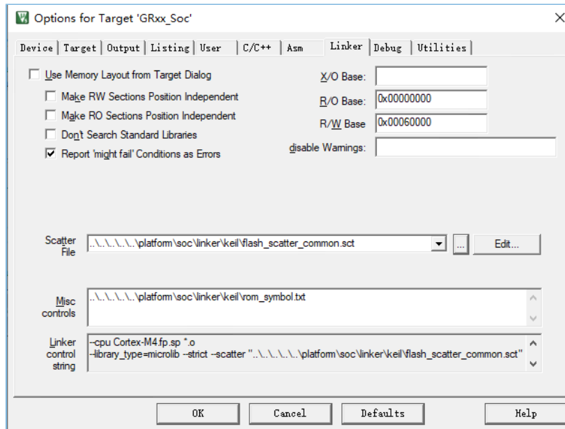
图 4-8 配置Scatter File
