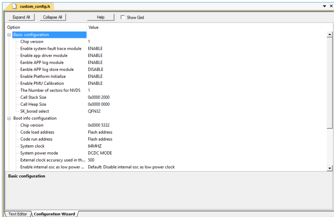
图 4-7 Configuration Wizard for custom_config.h
