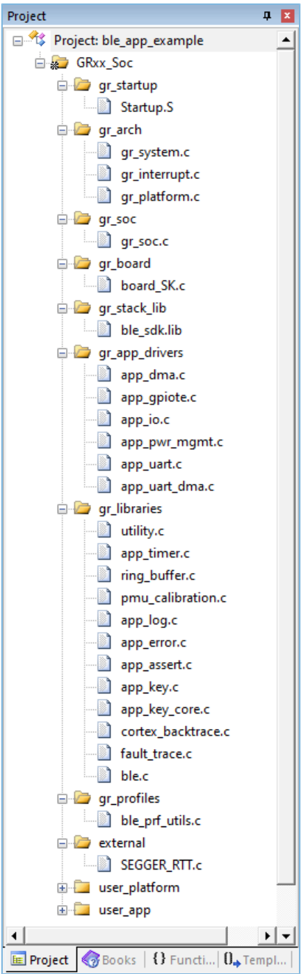
图 4-5 SDK groups
